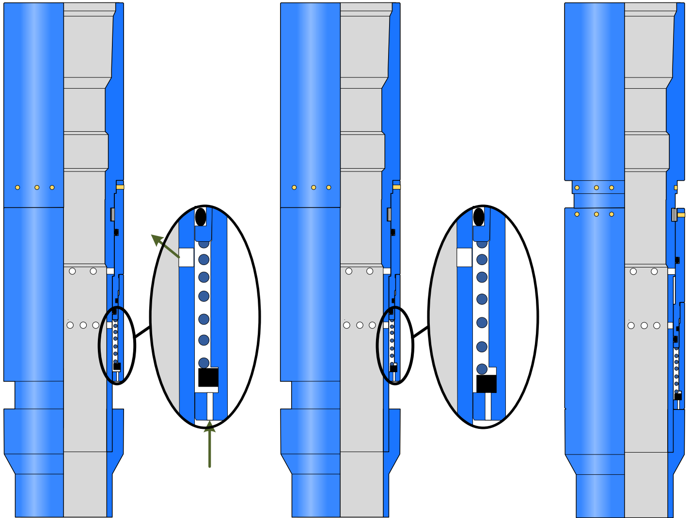
Automatic fill while running in the tubing string
